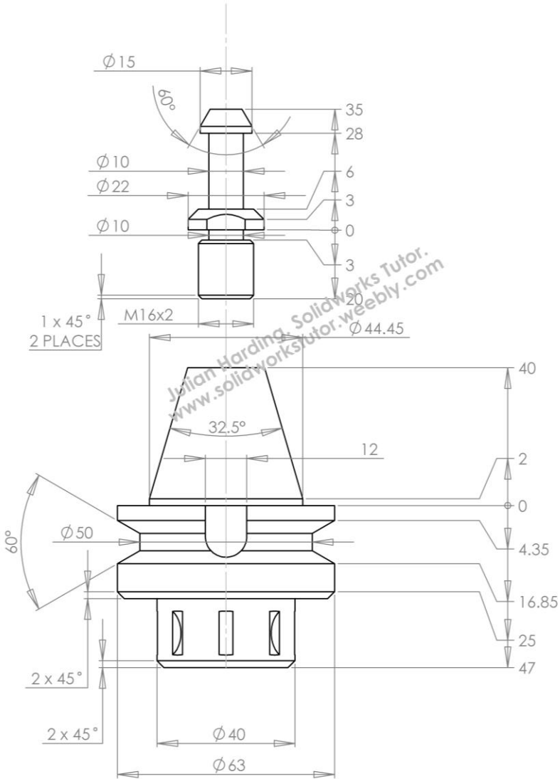
BT 40 Tool Holder Assambly.
